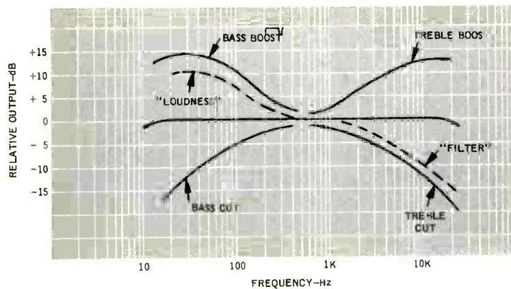
Fig. 8—Tone control, loudness, and high filter characteristics.
