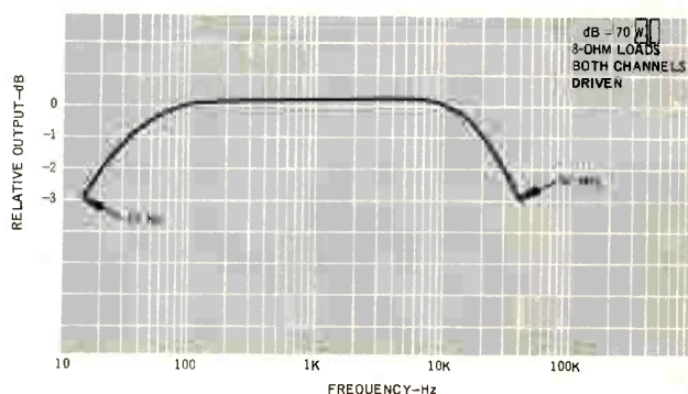
Fig. 6—Power bandwidth.
