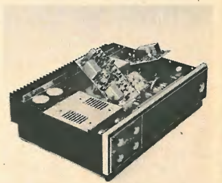
Hinged circuit boards for FM IF, AM IF, Multiplex and Phono Preamp sections — six plug-in boards for all other major circuitry.
