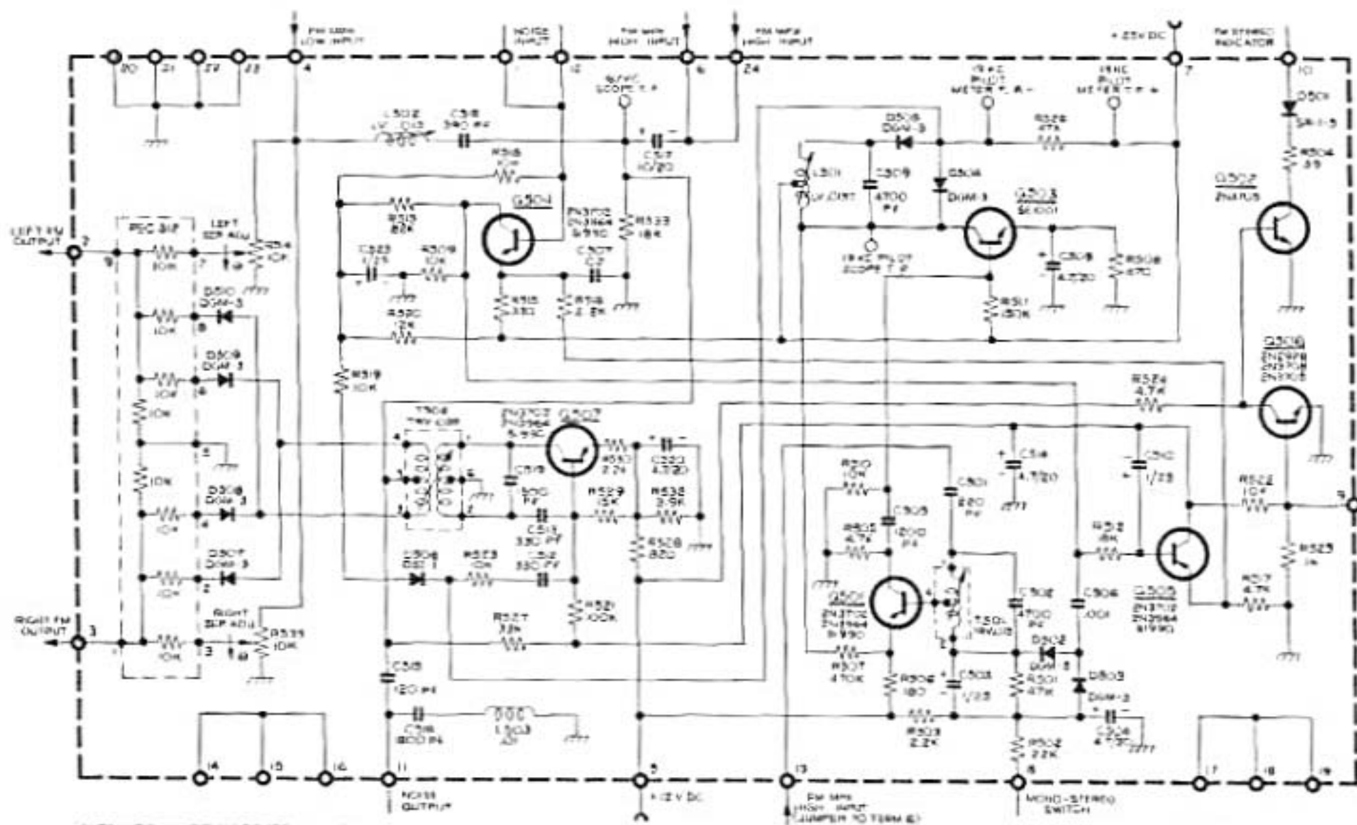
AUTOMATIC MULTIFLEX DEMODULATOR
